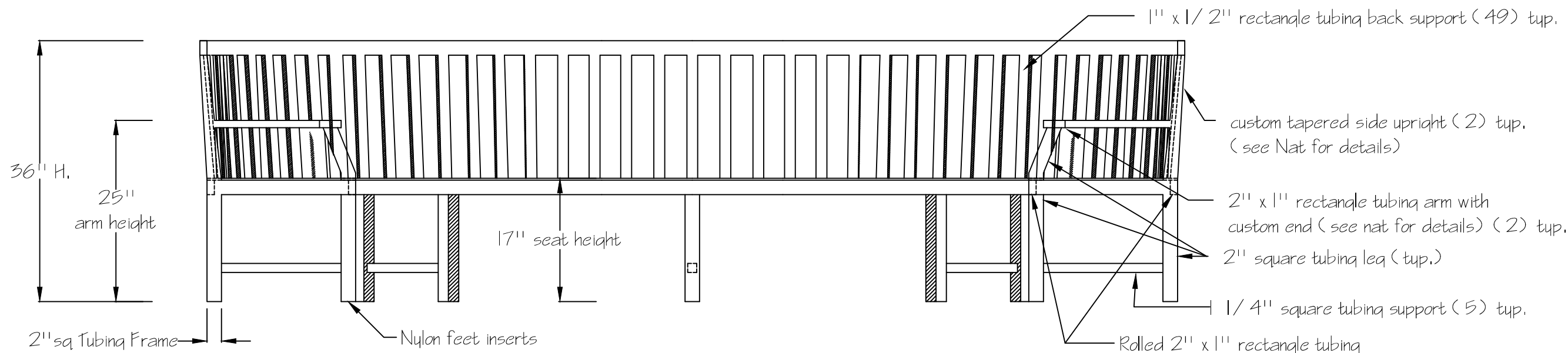
Elevation View
