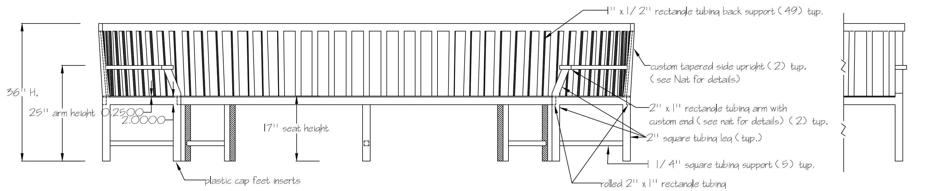
Elevation View
