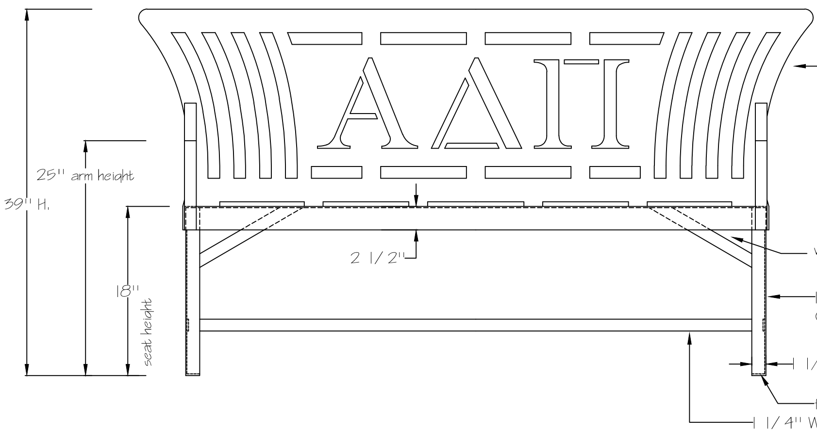
Front View
